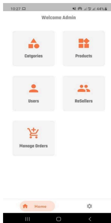
Figure 4: Main Page
