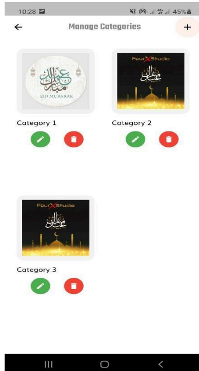
Figure 11: Manage categories
