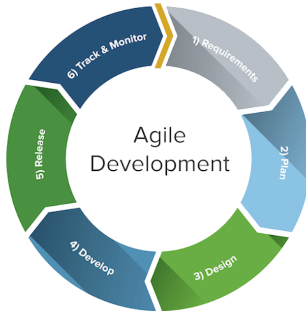
Figure 1: Agile Approach
