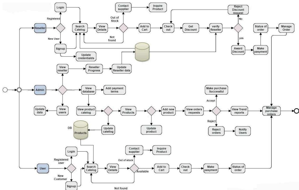
Figure 47: BPMN
