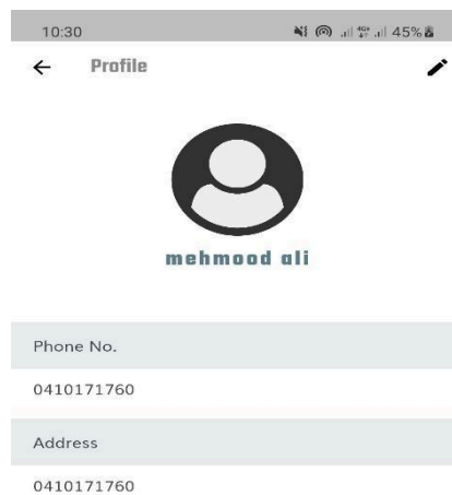
Figure 13: View Users
