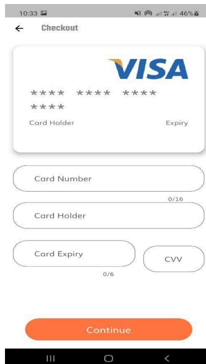
Figure 23: Checkout
