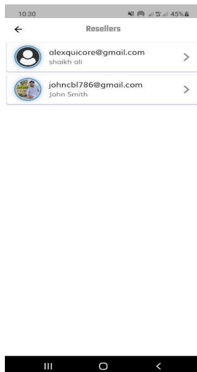
Figure 16: View resellers
