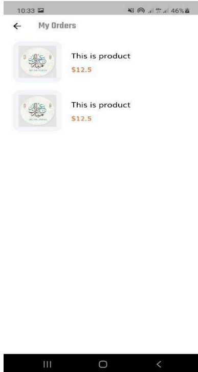
Figure 24: view Orders
