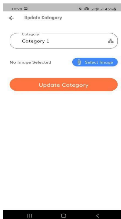
Figure 12: Update Categories
