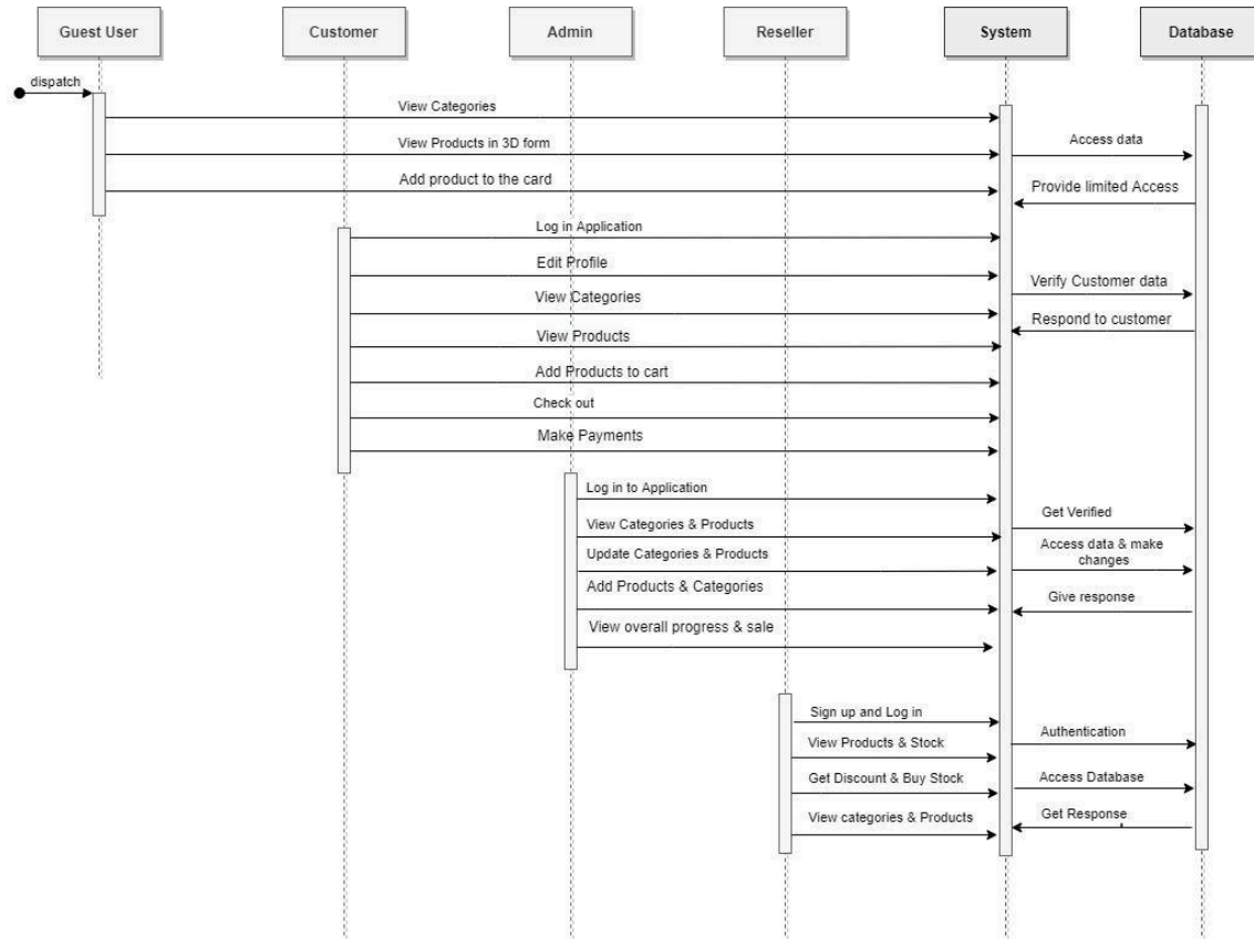
Figure 45: Sequence Diagram
