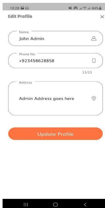
Figure 30: Update Profile
